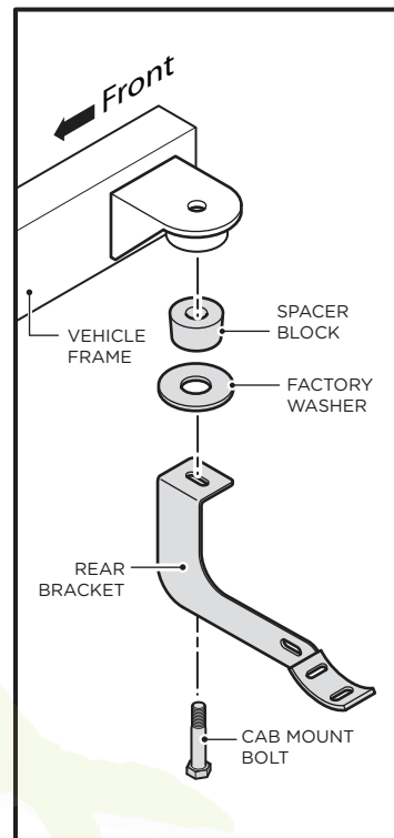
Rear Bracket
