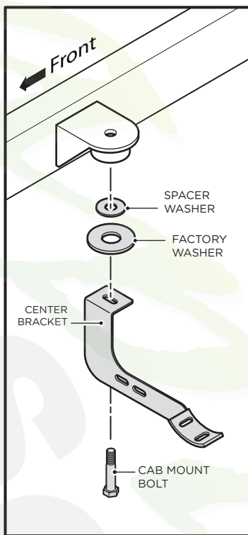
Center Bracket
