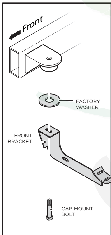
Front Bracket
