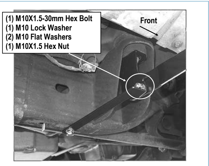
(Fig 7) Passenger Front Support Bracket Installation (For Up to 2007 2500/3500 Models)
