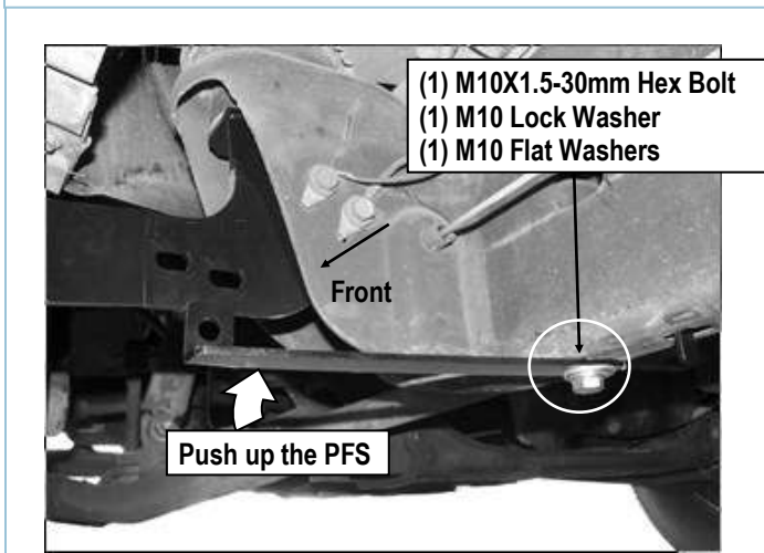
(Fig 6) Passenger Front Support Bracket Installation (For Up to 2007 2500/3500 Models)
