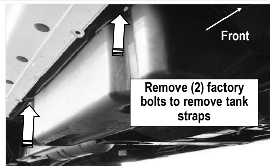
(Fig 11) 07-16 Passenger side DEF tank and cover
