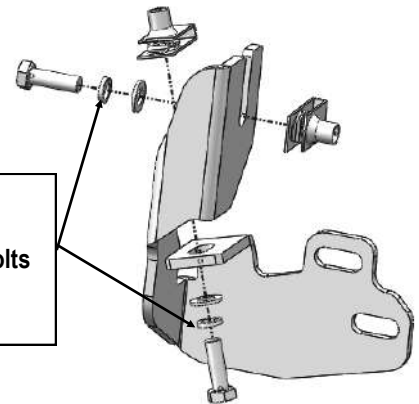
(Fig 12) Passenger Front Mounting Bracket Installed
