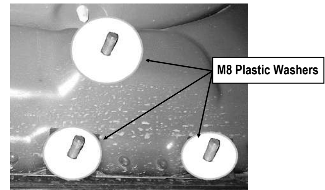
(Fig 2) Thread M8 Plastic Washers onto all mounting studs
