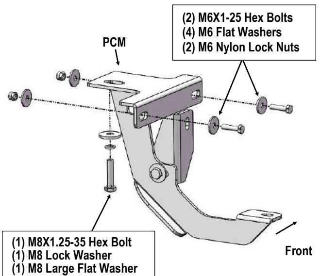
(Fig 5) Passenger Center Bracket Installed
