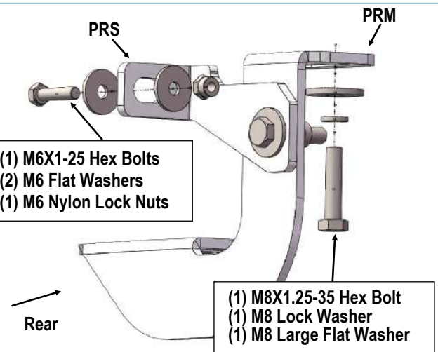
(Fig 8) Passenger Rear Bracket Installed
