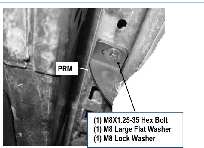
(Fig 16) Passenger Rear Mounting Bracket Installed
