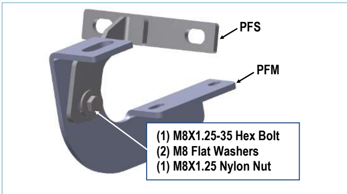
(Fig 6) Passenger Front Mounting Bracket Assembly
