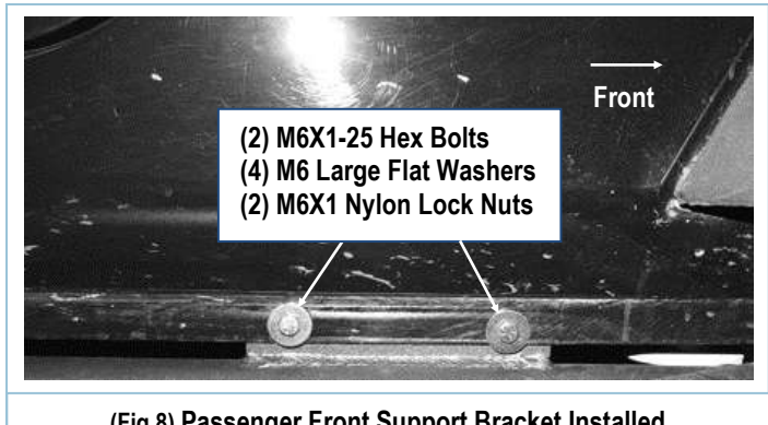
(Fig 8) Passenger Front Support Bracket Installed
