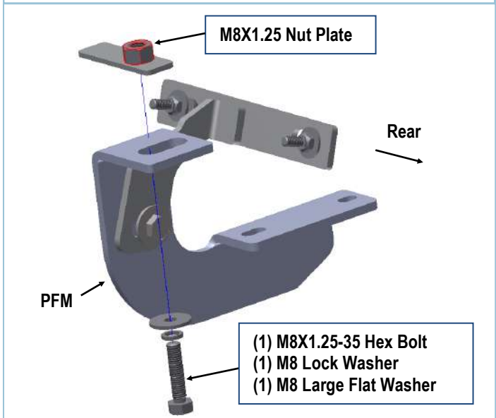
(Fig 9) Passenger Front Mounting Bracket Installed (Vehicles with open mounting location)
