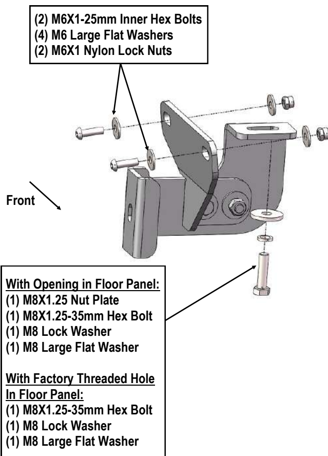
(Fig 7) Passenger Front Brackets Installation
