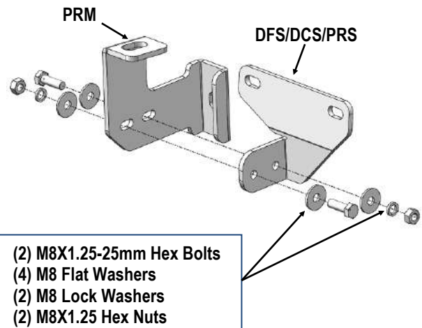
(Fig 5) Passenger Rear Mounting Bracket Assembly
