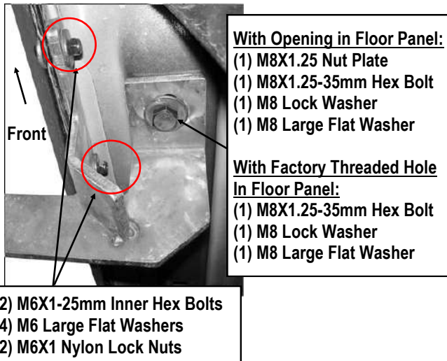
(Fig 6) Passenger Front Brackets Installation
