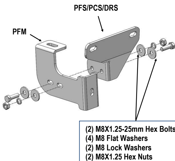
(Fig 3) Passenger Front Mounting Bracket Assembly
