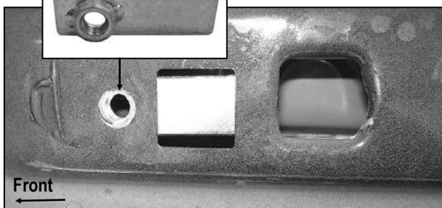
(Fig 1A) Driver Side Front Mounting Location (Vehicles with open mounting location)
