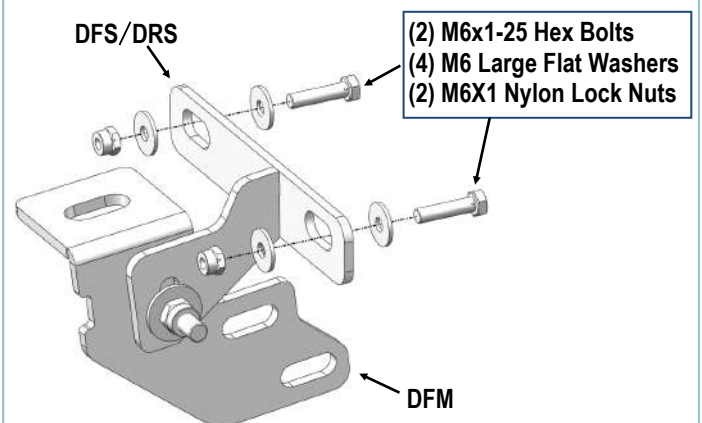
(Fig 9) Driver Front Support Bracket Installation
