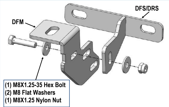
(Fig 6) Driver Front Mounting Bracket Assembly
