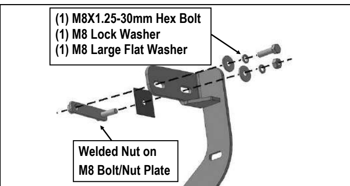
(Fig 6B) Secure Driver Front Mounting Bracket To the Welded Nut on M8 Bolt/Nut Plate
