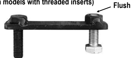
(Fig 3) Thread (1) M8X1.25-30 Hex Bolt into the welded nut on the plate.
