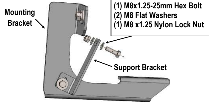
(Fig 14) Driver Support Bracket Installation
