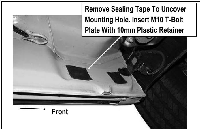
(Fig 1) Driver Front Mounting Bracket Location
