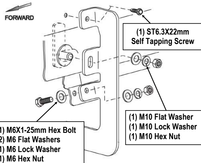
(Fig 4) Passenger Side Front Mounting Bracket Installation
