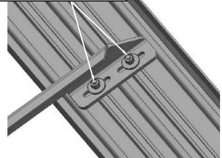
(Fig 8) Running Board Installed Onto Mounting Bracket
