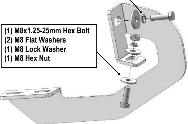
(Fig 3) Driver Front Mounting Bracket Installed
