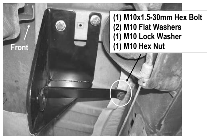
(Fig 4a) Passenger Front Support Bracket (PFS) Installation
