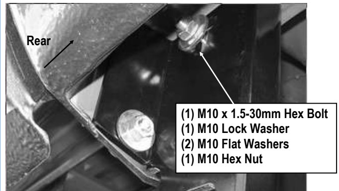
(Fig 7) Passenger Rear Mounting Bracket (PRM) Installation
