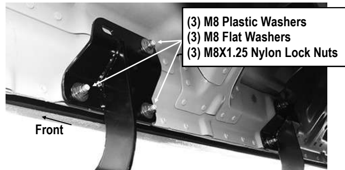
(Fig 3) Passenger Front Mounting Bracket Installed
