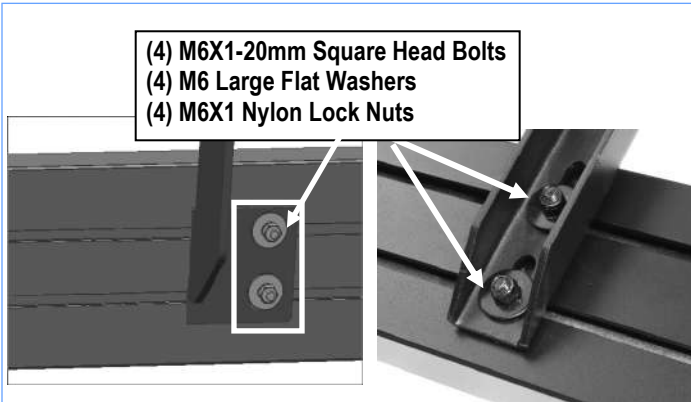
(Fig 14) Running Board Installed Onto Mounting Bracket
