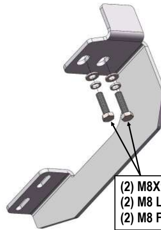
(Fig 2) Driver Front Mounting Bracket Installation
