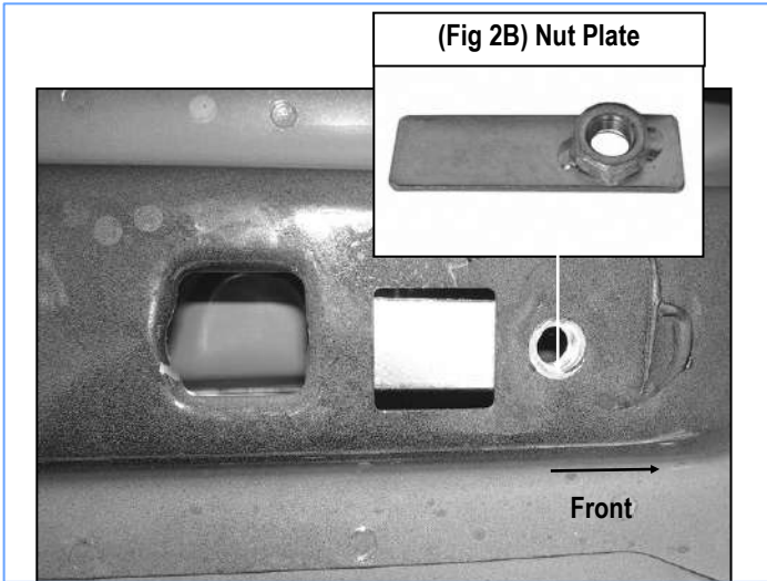
(Fig 2A) Driver Side Front Mounting Location (Vehicles with open mounting location)
