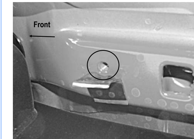
(Fig 3) Driver Side Front Mounting Location (Vehicles with factory threaded hole in floor panel)
