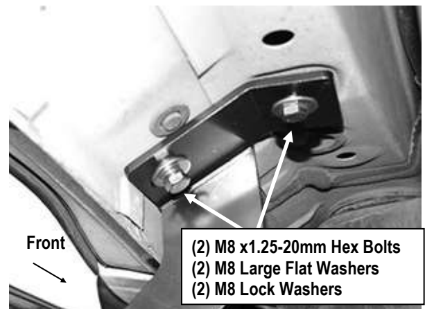
(Fig 2) Driver Side Front Mounting Bracket Installation
