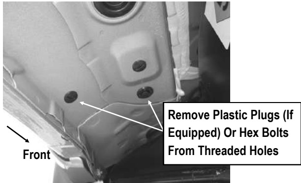
(Fig 1) Driver Front Mounting Bracket Location
