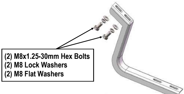
(Fig 4) Driver Center & Rear Mounting Bracket Installed
