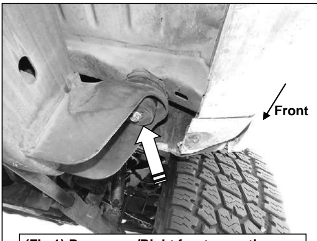
(Fig 1) Passenger/Right front mounting location. Temporarily remove the body bolt
