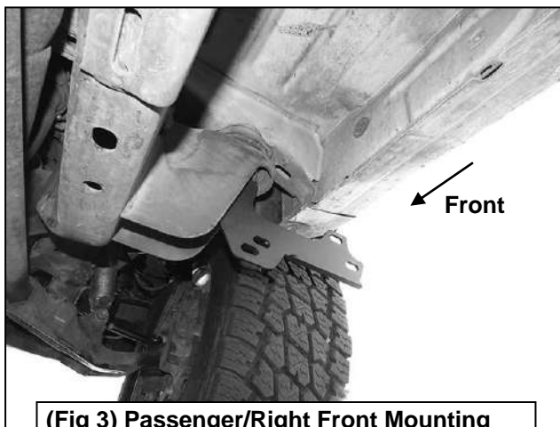
(Fig 3) Passenger/Right Front Mounting Bracket attached to the front body mount
