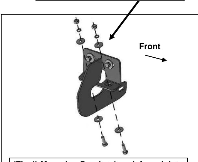
(Fig 4) Mounting Bracket (use left or right side) attached to pinch weld
