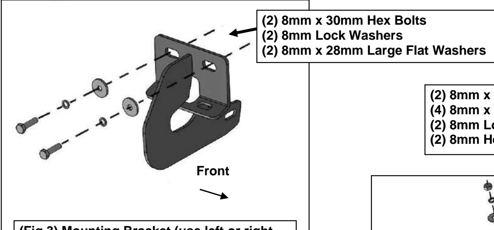
(Fig 3) Mounting Bracket (use left or right side) attached to inner body panel
