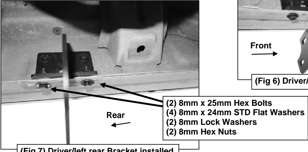
(Fig 7) Driver/left rear Bracket installed
