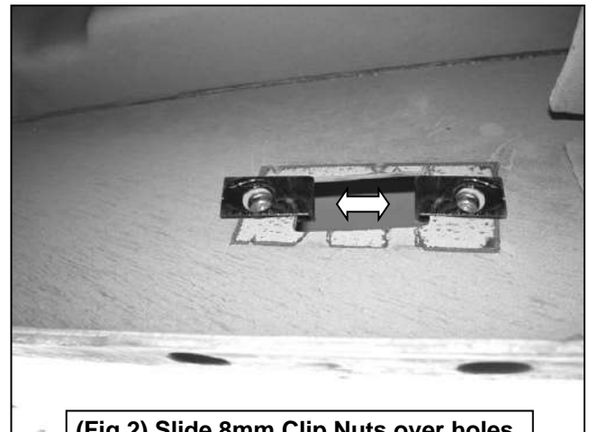
(Fig 2) Slide 8mm Clip Nuts over holes
