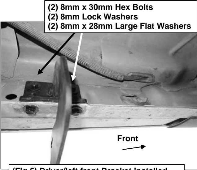
(Fig 5) Driver/left front Bracket installed
